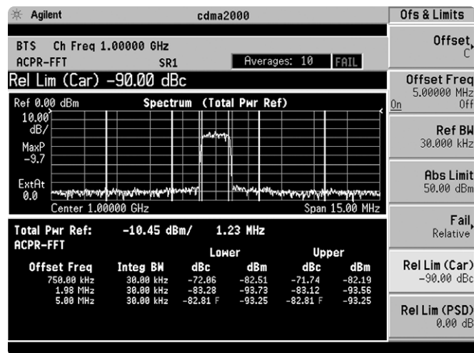
Figure 2. Multi-offset ACPR
